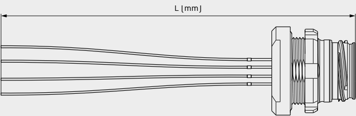
Panel mount receptacle (Style K) single wires..... 43
